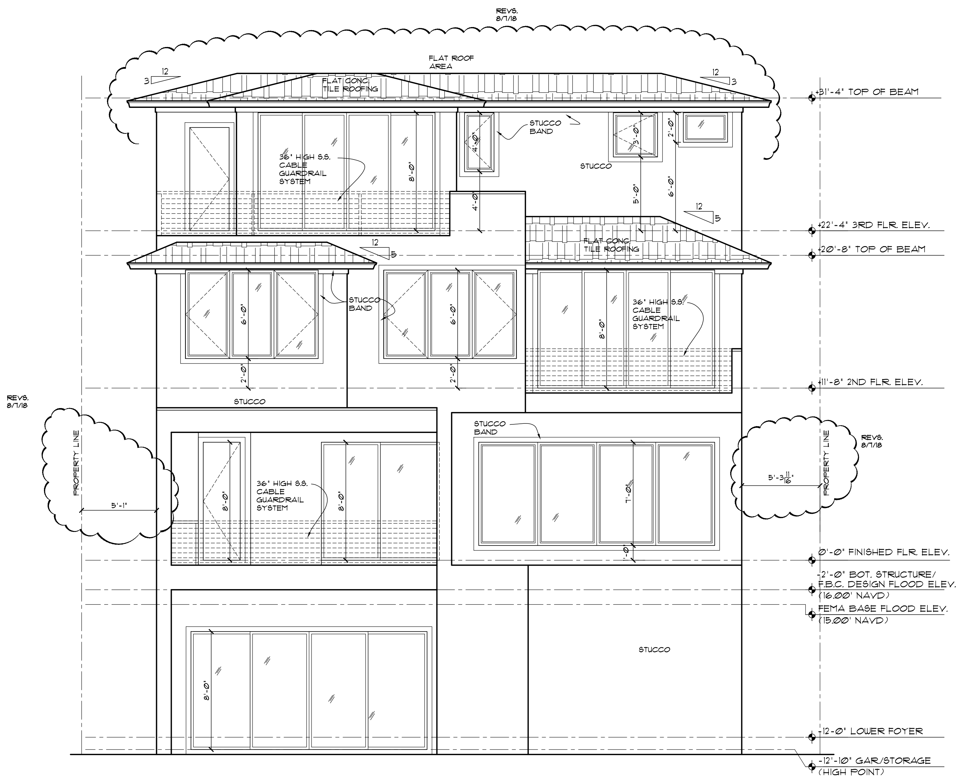
REAR ELEVATION SCALE: 1/4" = 1'-0"
